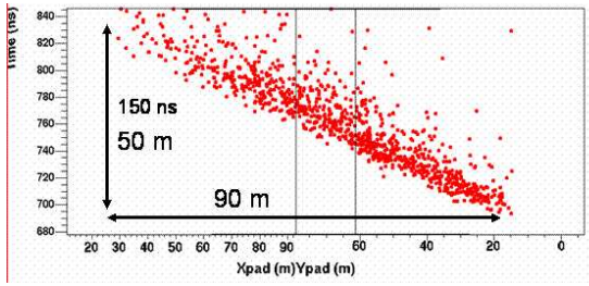
Figure 9: The time distribution vs X,Y on a shower event.
