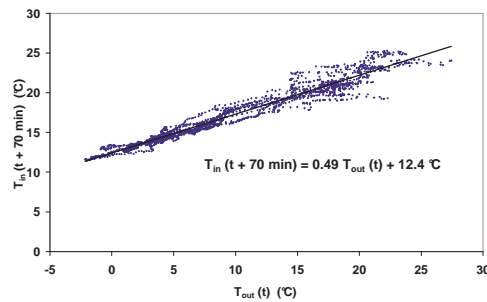
Figure 4: 70-minute time-delayed inner temperature near the carpet center versus the outer temperature, related to the May 2007 monitoring data. The result of the linear fit is also shown.
