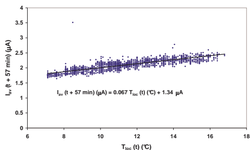
Figure 8: Correlation plot of the 57-minute delayed average RPC current and the local temperature for one ARGO-YBJ cluster near the carpet center (Cluster 91). The result of the linear fit is also shown.
