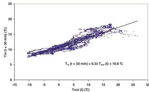
Figure 3: 30-minute time-delayed inner temperature near the carpet center versus the outer temperature, related to the February-March 2007 monitoring data. The result of the linear fit is also shown.
