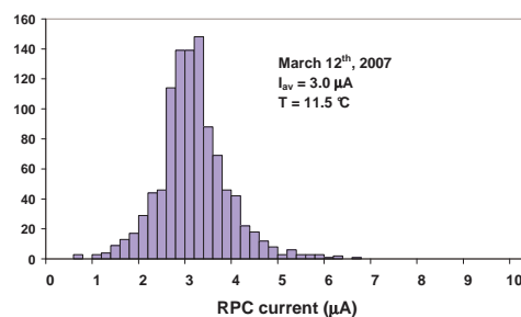
Figure 7: Single-chamber current distribution for 1400 RPCs of the ARGO-YBJ carpet.
