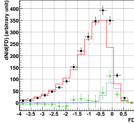
Figure 2: Fisher Discriminant distribution. The closed circles indicate those for on-source events. The solid and dotted histogram are the best-fit FD distributions for background events and for MC gamma-ray events, respectively. The closed squares show the background subtracted gamma-ray candidate events.
