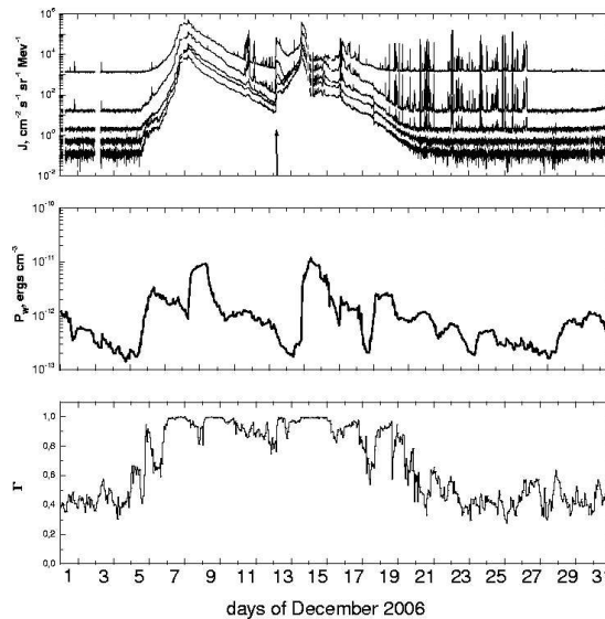
Figure 3: From top to bottom: 5-min fluxes from 5 CR channels, energy density of MHD-waves and coherence between 4-th and 5-th channels in measuring of cosmic rays aboard the ACE spacecraft. The arrow shows the GLE event.
