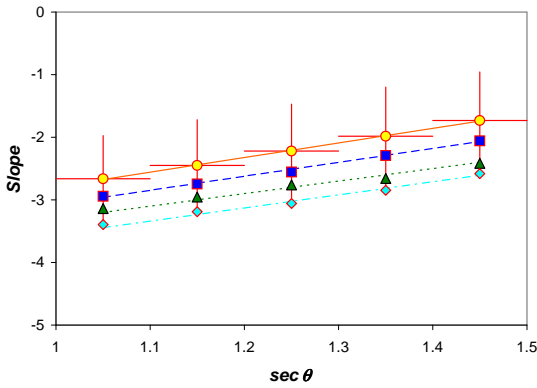
Figure 1: Average slope of lateral distribution function of charged particles as a function of zenith angle and energy. The data are sampled in five \sec \theta intervals shown by horizontal bars; energy bins (in EeV) are: (1, 1.78) - circles; (1.78, 3.16) - squares; (3.16, 5.62) - triangles; (5.62, \infty ) - rhombuses; RMS slope errors in bins are shown by vertical bars; approximation lines have d\eta/d\sec \theta = 2.15 \pm 0.15 .
