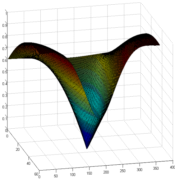
Figure 2: Normalized geomagnetic force on secondary particles on an EAS event in different \theta and \phi .
