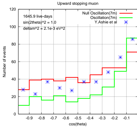
Figure 5: Zenith angle distribution for Upward Stopping Muon events for 1645.9 live days
