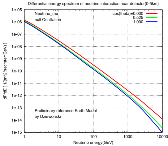
Figure 1: The interaction energy spectrum without neutrino oscillation
