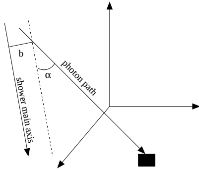
Figure 1: Reconstruction variables
