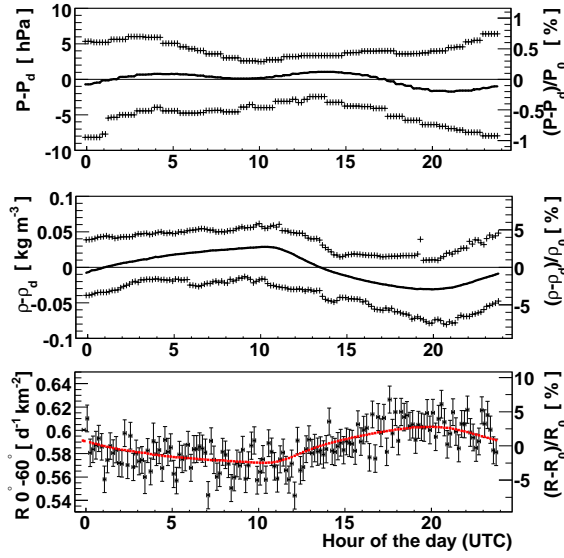
Figure 2: Variation of P (top) and \rho (middle) during the day: the values averaged over 2005 and 2006 (lines) are shown together with the maximum variation values during the 2 years considered (crosses). Bottom: the result of the fit (red) reproduces very well the average diurnal modulation of the measured rate (black). The local time is UTC - 3 h
