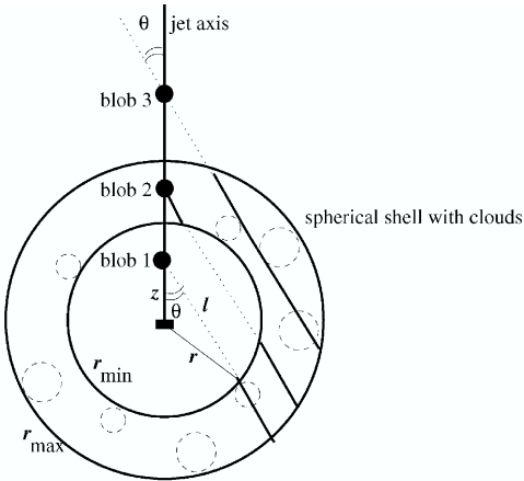
Figure 1: The schematic representation of a model of the Broad Line Region. The drawing is taken from [5].
