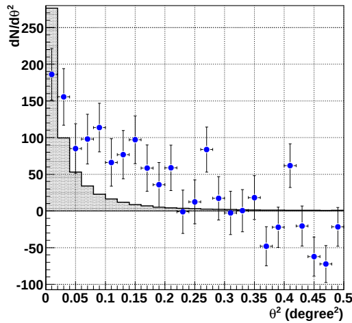
Figure 2: Preliminary \theta^2 distributions for HESS J1303–631 using the FD method with fitted FD distribution. The closed circle is those for on-source events. The hatched histogram shows point spread function normalized to give the same number of ON-source events in \theta^2 < 0.06 .
