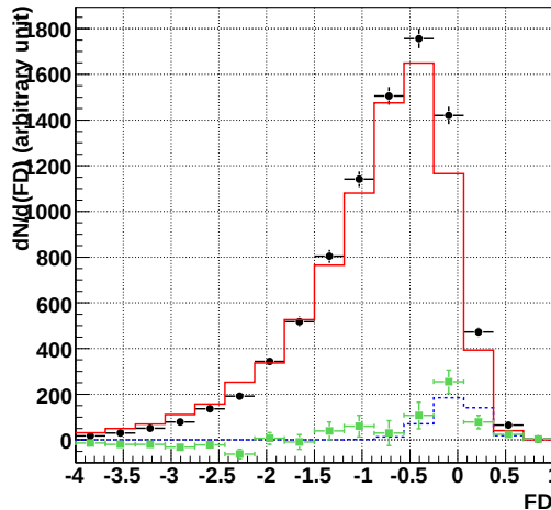
Figure 1: Preliminary Fisher Discriminant (FD) distributions for HESS J1303–631. The closed circle and square are those for on-source events and the background subtracted gamma-ray candidate events. Solid and dotted histogram are the best-fit FD distributions for background events and for MC gamma-ray events.
