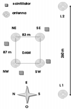
Figure 1: CODALEMA array on Jan 15 th 2005.
