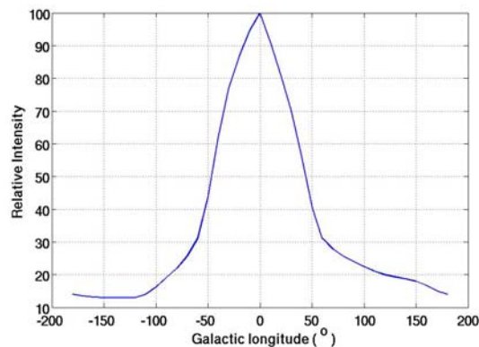
Figure 7: Radio signal intensity along the galactic plane [3].
