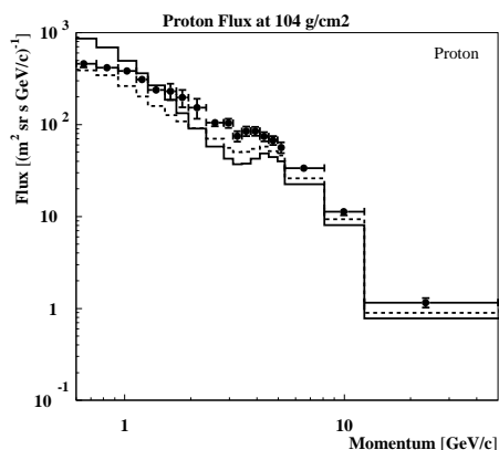
Figure 2: Same as figure 1 but for an altitude of 104 g/cm 2 .
