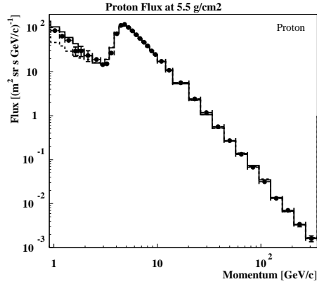
Figure 1: Absolute proton flux versus momentum, at an altitude of 5.5 g/cm 2 . The solid circles correspond to CAPRICE98 data, while the histograms represent AIRES simulations using the A1 (dashed line) and A2 (solid line) codes.
