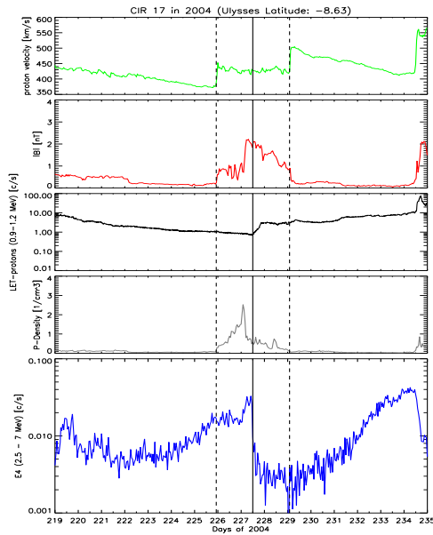
Figure 4: Same parameter as in Fig. 3 but for the time period around day 227 in 2004.
