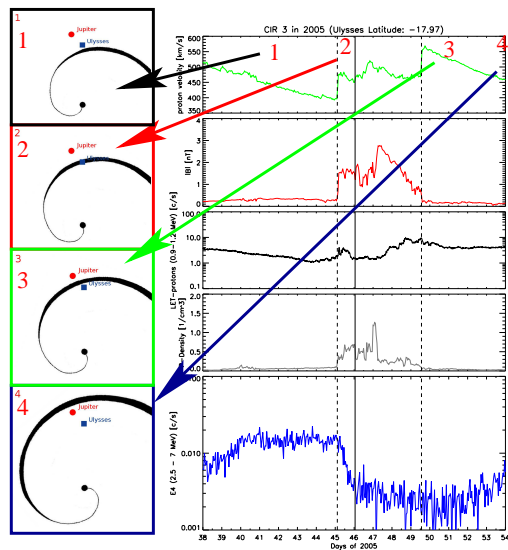
Figure 3: (1) to (4) sketch of different position of a corotating interaction regions (CIRs) with respect to the position of Jupiter and Ulysses; adapted from Conlon and Simpson [3]. On the right side hourly averaged solar wind speed, magnetic field strength, 0.9-1.2 MeV protons, solar wind density and 2.5-7 MeV electrons.
