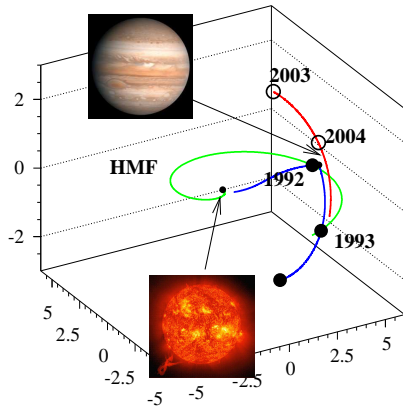
Figure 1: Sections of the Ulysses trajectory from launch to 1994 (blue curve) and from 2003 to 2005 (red curve) in a coordinate system where the positions of Jupiter and Sun are fixed. A Parker magnetic field line in Jupiter's orbital plane is shown for a solar wind speed of 400 km/s. Circles are plotted at the beginning of each year.
