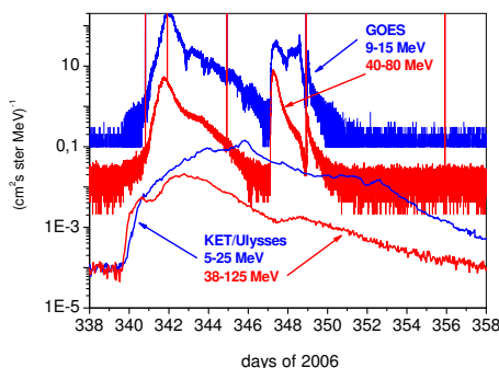
Figure 3: Comparison of ~10 MeV and ~50 MeV proton intensities measured by KET/ Ulysses (hourly average) and GOES EPS (5-min average) in December 2006.
