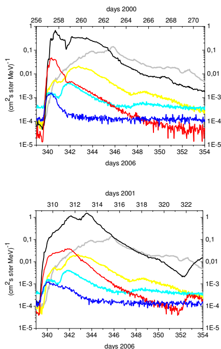
Figure 4: Comparison of KET time profiles (grey – 5-25 MeV; yellow – 38-80 MeV; cyan 80-125 MeV) measured in December 2006 with those in September 2000 and November 2001 (black, red and blue curves).
