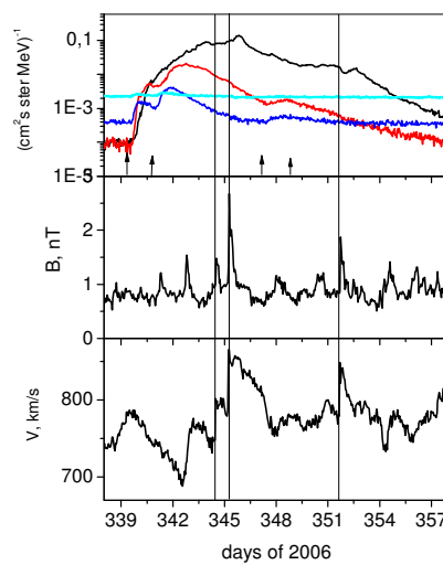
Figure 1: From top to bottom are presented KET/ Ulysses proton intensities within energy bands 5 – 25 MeV (black), 38-125 MeV (red), 125-250 MeV (blue) and 250-2000 MeV (cyan); magnetic field strength (VHM/FGM) and solar wind velocity (SWOOPS). Black arrows mark X-class solar flares on days 339, 340, 347 and 348 (2006 December 5, 6, 13 and 14) [1]; vertical lines indicate the shock arrivals on days 344, 345 and 351, respectively [4].
