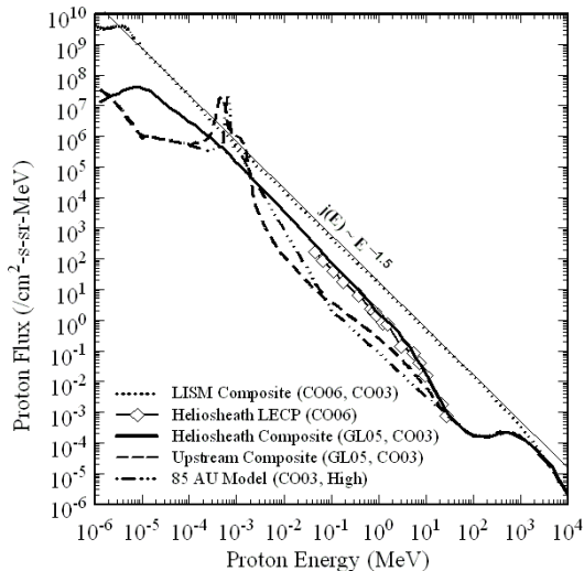
Figure 3. Composite proton flux spectra at plasma to cosmic ray energies upstream of the solar wind termination shock (GL05 [15], CO03 [19]), in the inner heliosheath (GL05 [15], CO06 [14]) and as projected with the E^{-1.5} spectrum (CO06 [14]) for the local interstellar medium (LISM).
