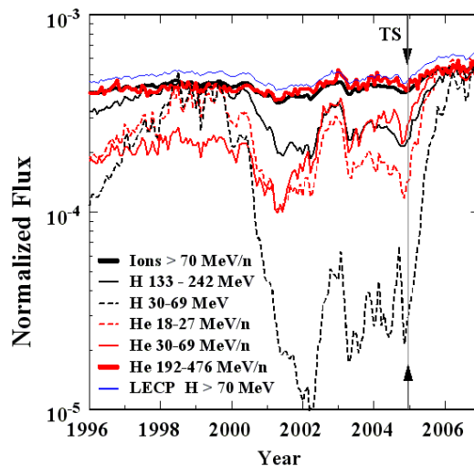
Figure 1: Fluxes and count rates for cosmic ray protons and helium over the past decade as measured by the Cosmic Ray (CRS) and Low Energy Charged Particle (LECP) experiments on Voyager 1. Each time profile (black and red respectively for CRS proton and alpha fluxes as 26-day averages, blue for LECP proton fluxes as daily averages) is roughly normalized to the peak intensities in the rise to solar minimum during 2006. “TS” and the vertical line denote the date of the termination shock crossing, Dec. 16, 2004.
