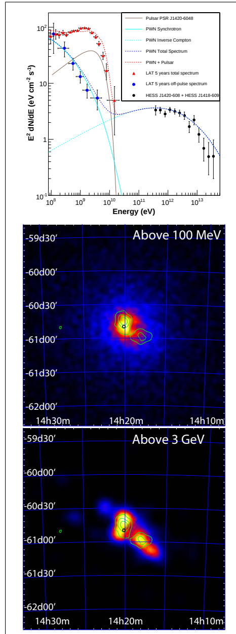
Figure 2: Top: Spectral Energy distribution for the Kookaburra region, containing a simulated Pulsar and PWN in the GLAST range and the VHE gamma-ray measurements by H.E.S.S. [8]. Center: Corresponding GLAST gamma-ray image simulated as above for energies > 100 MeV, and Bottom: > 3 GeV).
