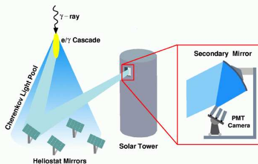
Figure 1: The showerfront-sampling technique as employed by STACEE. Cherenkov light from air shower cascades is reflected by the heliostat mirrors onto secondary mirrors in the receiver tower, which in turn concentrate the light onto a bank of photomultiplier tubes.
