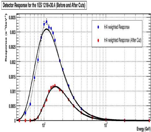
Figure 3: Energy response curves of the STACEE detector before and after quality cuts, for a differential photon spectral index of -3.0 . The energy threshold of STACEE is defined by the peak of the response curve, although STACEE is sensitive to lower energies.
