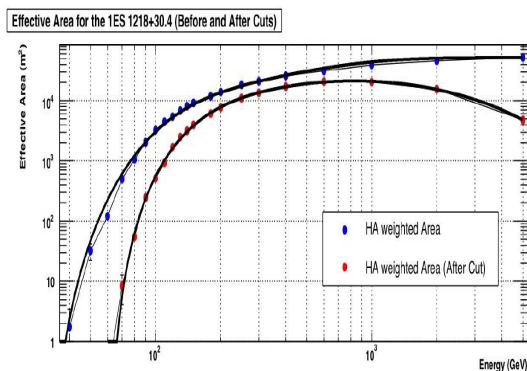
Figure 2: Hour-angle weighted effective area of the STACEE detector for the 1ES 1218+304 observations. The lower plot shows the effective area after quality cuts.
