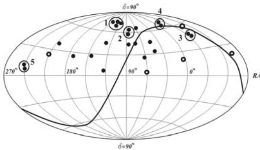
Fig.1. Distribution of showers without muons (closed circles) and depleted in muon (open circles) in the equatorial coordinates, declination \delta and right ascension, RA. Large circles denote clusters 1-5. Big circles – clusters.
