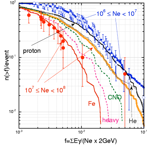
Figure 2: Distribution of family energy normalized by N_e \times 2 \text{ GeV} , f \equiv \sum (E_\gamma + E_h(\gamma)) / (N_e \times 2 \text{ GeV}) . Circles are for the experimental data and lines are for simulated events. Open circles and line are events of 10^6 \leq N_e < 10^7 and solid circles and dotted line for 10^7 \leq N_e < 10^8 . Thick lines are for the case of proton-dominant composition shown in Table 1.
