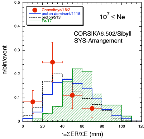
Figure 3: Distribution of average lateral spread \langle ER \rangle of \gamma -rays in the families associated with air-showers of 10^7 \leq N_e < 10^8 . Circles are experimental data and lines are simulated data for proton primaries (dash-dotted), iron-primaries (shaded) and all particles with spectrum.
