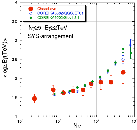
Figure 1: Diagram on air-shower size, N_e , and average energy sum, \langle \log \sum E_\gamma \rangle , of accompanied families.
