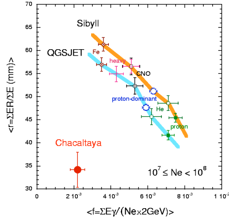
Figure 4: Diagram on average family energy normalized by shower size and average lateral spread, for the events with 10^7 \leq N_e < 10^8 .
