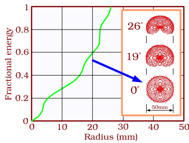
Figure 2: Optical spot (produced by paraxial beams) on mosaic surface with mosaic shadow
