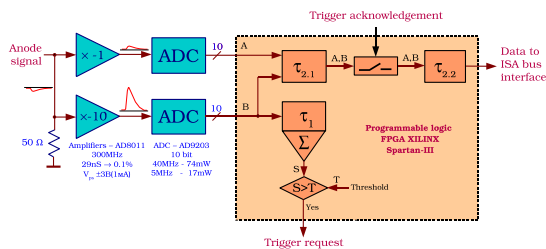
Figure 5: Block scheme of channel
