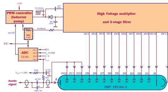
Figure 3: High voltage power supply for optical module
