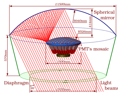
Figure 1: Optical scheme of SPHERE-2 detector (without mosaic shadow)
