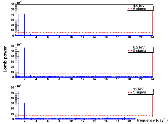
Figure 2: Lomb Power of the frequency \text{day}^{-1} between 2 years and 1 hour for Tibet III Air Shower Array data for different representative energies: (Up) 4.0TeV, (Middle) 6.2TeV, (Bottom) 12.0TeV. The 5\sigma is shown by red broken line.
