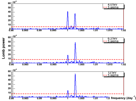
Figure 1: Lomb power of the frequency \text{day}^{-1} around solar diurnal day for Tibet III Air Shower Array experimental data for different representative energies: (Up) 4.0TeV, (Middle) 6.2TeV, (Bottom) 12.0TeV. The 5\sigma is shown by red broken line.
