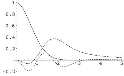
Figure 5: Integrated Molière terms, F^{(0)}(\vartheta) (solid line), F^{(1)}(\vartheta) (broken line), and F^{(2)}(\vartheta) (dot line).
