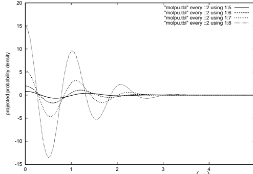
Figure 4: Molière series function f_P^{(n)}(\varphi) with n from 3 to 6, for projected angular distribution.
