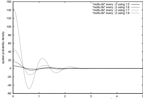
Figure 3: Molière series function f^{(n)}(\vartheta) with n from 3 to 6, for spatial angular distribution.
