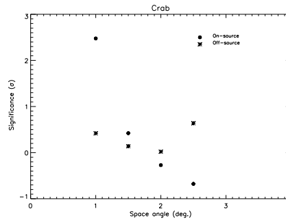
Figure 2: Significance as function of space angle
