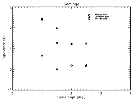
Figure 2: Significance as function of space angle for Geminga pulsar
