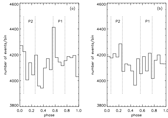
Figure 1: Phase histogram of Geminga pulsar events for (a) Mattox et al. and (b) Jackson et al. ephemeris
