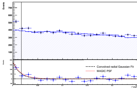
Figure 1: Distributions of \theta^2 (in degrees). In the lower panel shows the \theta^2 distribution after background subtraction. The excess number is obtained for events with \theta^2 below a selection cut (vertical line). The red Gaussian curve is the telescope PSF. The black curve is the result of a Gaussian fit and limits the extension of the source.
