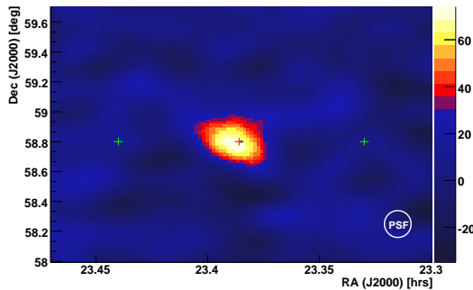
Figure 2: Sky Map of Cas A region. A cut in SIZE of 400 p.e. was applied: the green crosses are the 2 wobble positions; the black cross is the HEGRA c.o.g.; the red cross is the MAGIC c.o.g.
