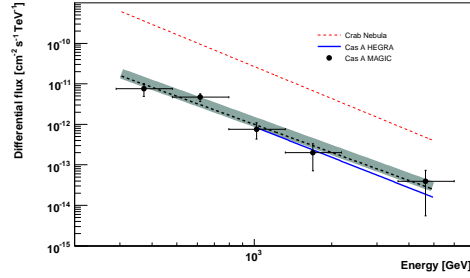
Figure 3: Cas A spectrum above 250 GeV. The blue line represents the earlier measurement by HEGRA. The red line represents the Crab nebula spectrum. The shaded area is the 1\sigma statistical error of the fit.
