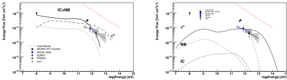
Figure 4: Cas A spectrum energy distribution as measured by MAGIC. The shaded area is the 1\sigma statistical error range, under the assumption of power law spectrum. Whipple, EGRET and CAT upper limits and the HEGRA spectrum are also indicated. On the left, the MAGIC and HEGRA spectra compared with the model in [5]. Gamma-ray fluxes from Inverse Compton (IC) plus nonthermal Bremsstrahlung (NB) for different model parameters are shown with black and grey solid lines. The \pi^0 -decay (dotted) \gamma -ray energy flux is shown with dotted-dash line. On the right, the MAGIC and HEGRA spectra are compared with the model in [7]. Both, hadronic and leptonic \gamma -ray emission are shown
