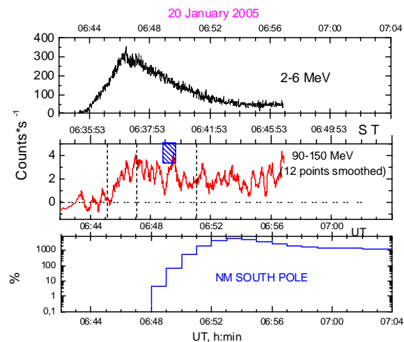
Figure 1: Gamma emission time profiles observed by the SONG (upper panels) and GLE measured by South Pole NM (lower panel). The time scale between the
