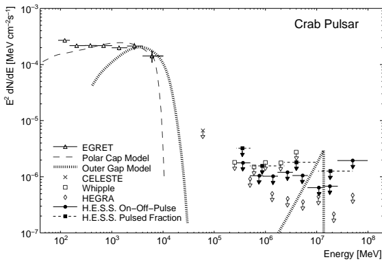
Figure 3: H.E.S.S. energy flux limits (99% c.l.) for pulsed emission of the Crab pulsar. The full circles and full squares correspond to the on-off-pulse and pulsed fraction limit determination methods, respectively. Below energies of 0.5 TeV the results were obtained with the low energy selection cuts, otherwise the standard cuts were used. The indicated polar cap curve was generated according to [10] and the outer gap model curve taken from [7]. Note that the southern location of H.E.S.S. allows only observations at rather high zenith angles for Crab, prohibiting a deep exposure especially at low energy thresholds.
