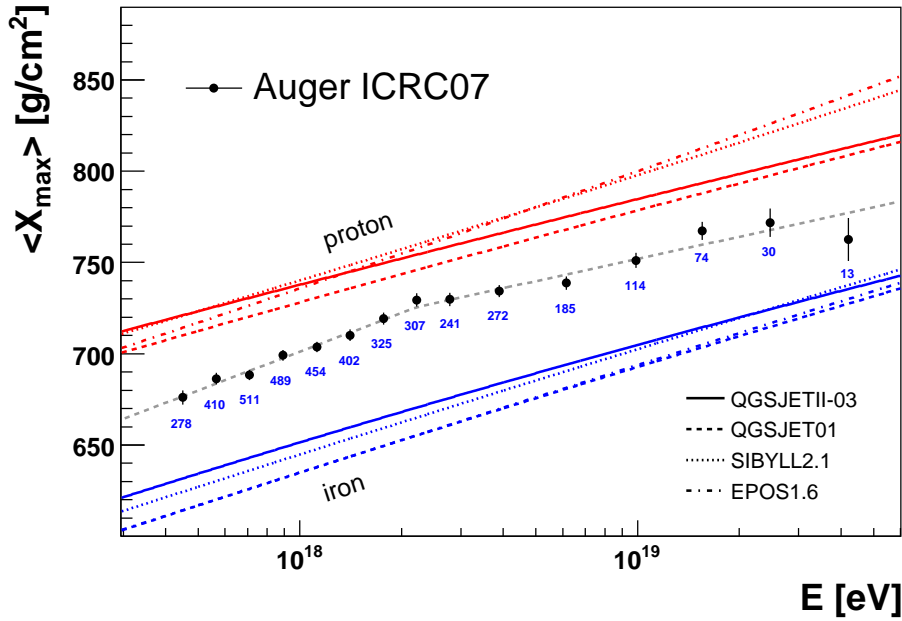
Figure 3: \langle X_{\max} \rangle as a function of energy compared to predictions from hadronic interaction models. The dashed line denotes a fit with two constant elongation rates and a break-point. Event numbers are indicated below each data point.
