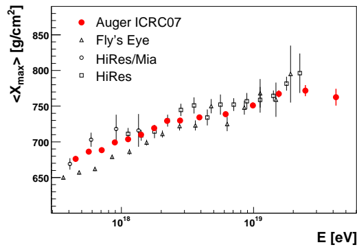
Figure 5: \langle X_{\max} \rangle as a function of energy compared to previous experiments.
