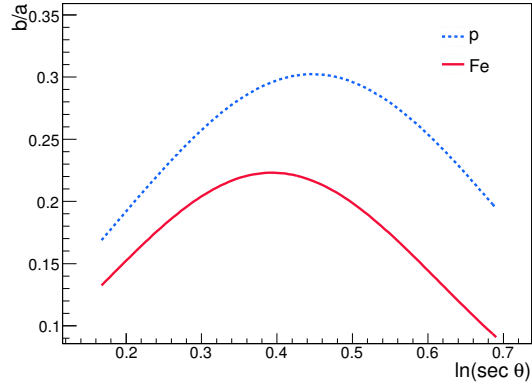
Figure 4: Development of the asymmetry factor in the risetime with zenith angle. The primary energy is \sim 10^{18.5} \text{ eV} .
