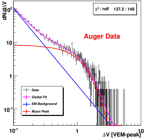
Figure 3: Distribution of jumps for Auger events with energy between 8-12 EeV and 40-50°, averaged over 251 stations - 100 showers - within the same core distance interval.
