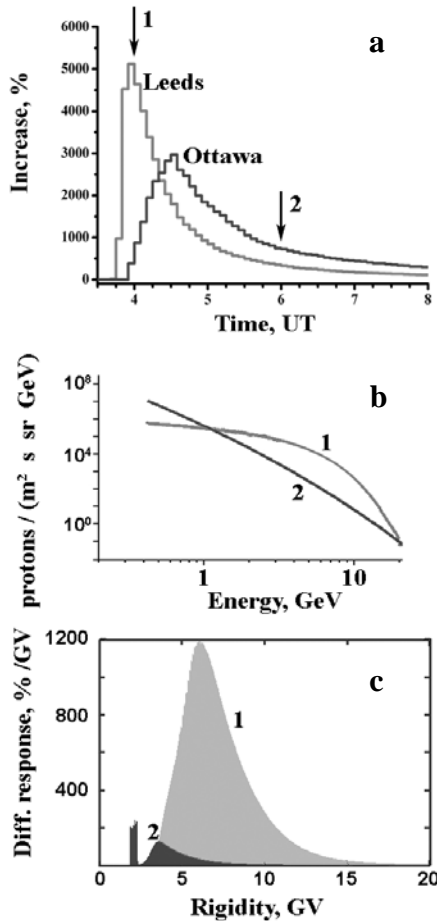
Fig.1. Intensity-time profiles at the Leeds and Ottawa neutron monitors (a), energy spectra derived at the moments 04:00 (1) and 06:00 (2) UT (b), and differential responses (c) of the Leeds neutron monitor to the exponential spectrum at the moment 1 (gray shading) and at the moment 2 to the power-law spectrum (black shading). By numbers are marked, respectively, the moments when the prompt component (1) or delayed one (2) were dominating. One can see comparable responses of both neutron monitors to the power-law spectrum.
