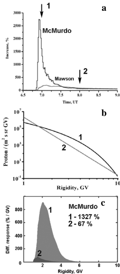
Fig.2. Intensity-time profiles at the McMurdo and Mawson neutron monitors (a), energy spectra derived at the moments 07:00 (1) and 08:00 (2) UT (b), and differential responses (c) of the McMurdo neutron monitor to the exponential spectrum at the moment 1 (gray shading) and to the power-law spectrum at the moment 2 (dark shading). One can see comparable responses of both neutron monitors to the power-law spectrum.
