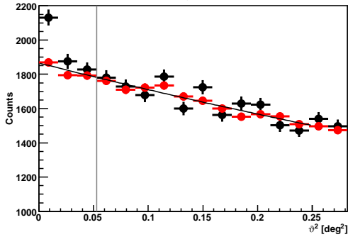
Figure 1: Distribution of the squared angular distance ( \vartheta^2 ). The black points represents \vartheta^2 with respect to the position of 1ES 1218+30.4.
