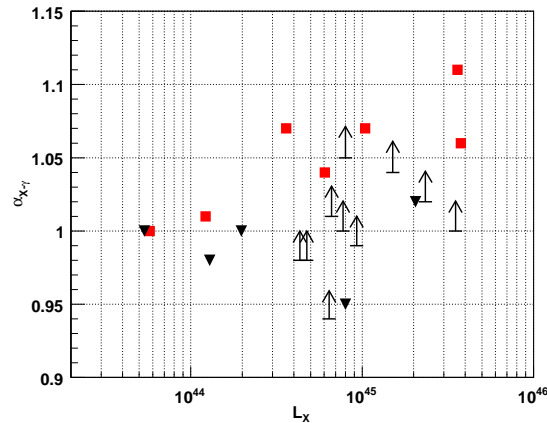
Figure 2: Overall spectral index \alpha_{X\gamma} vs. X-ray luminosity at 1 keV. The black triangles mark the detected TeV sources of the sample, while the red squares are all other TeV HBLs. The arrows indicate the u.l. presented in this work.
