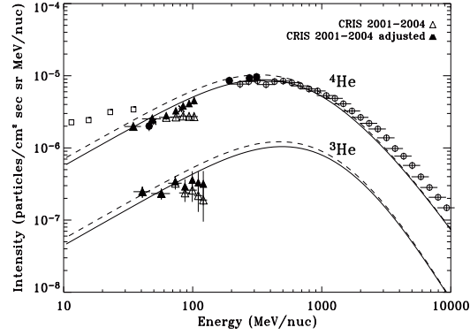
Figure 4: CRIS helium intensities during solar maximum conditions (Jan. 1 2001 to Jan. 1 2004) compared with the results from previous and concurrent experiments and results from GALPROP with an assumed \phi of 1100 & 1200 MV.
