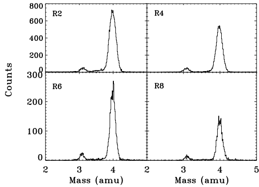
Figure 1: Mass histograms for helium in 4 energy ranges R2: 34-47 MeV/nuc, R4: 64-83 MeV/nuc, R6: 91-109 MeV/nuc, and R8: 113-131 MeV/nuc observed during solar minimum.
