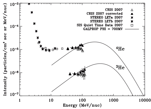
Figure 5: CRIS helium intensities during recent solar minimum conditions (Jan. 1 2007 to April 15 2007) compared with the results from concurrent observations of ACE/SIS (open squares), [14] (asterisks). Also shown are the predictions from GALPROP with \phi = 700 MV.
