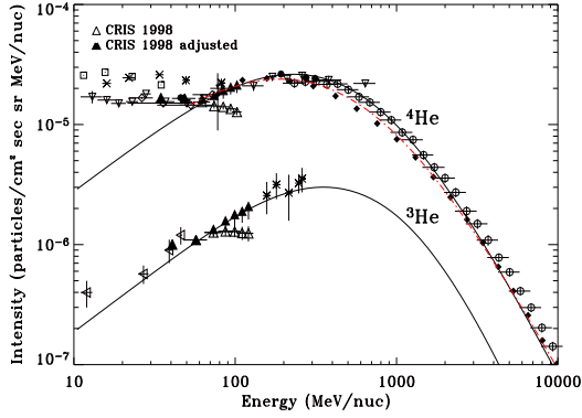
Figure 3: CRIS helium intensities during solar minimum conditions (Jan. 1 1998 to Jan. 1 1999). Observations include [16] (open circles), ACE/SIS (open squares), [2] (upside-down triangles), [1] (solid diamonds), [10] (asterisk), [12] (thick asterisk and open diamonds), [11] (solid circles). Also shown are the GALPROP results with \phi = 500 MV.
