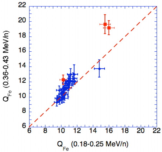
Fig. 3: Mean ionic charge of Fe for 35 interplanetary shock related SEP events.
