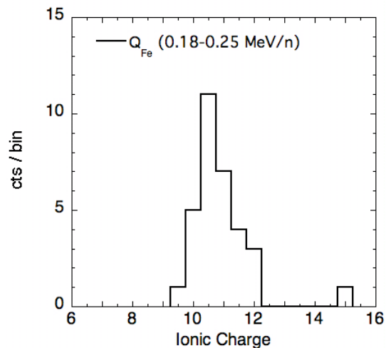
Fig. 2: Distribution of Fe charge states in the energy range 0.18-0.25 MeV/nuc.
