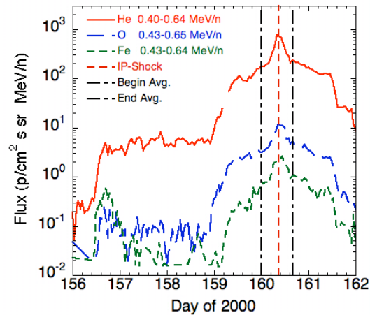
Fig. 1: Example of averaging time period including an interplanetary shock related intensity increase of He, O, and Fe.
