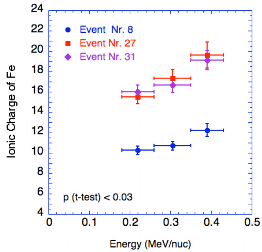
Fig. 4: Average ionic charge of Fe for the three events of this study with significant energy variation.
