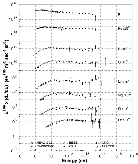
Figure 4: Intensities of individual ions measured by some experiments [10, 14, 11] in the energy interval 10^{10} - 10^{15} eV.
