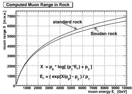
Figure 1: Calculated average muon range in standard and Soudan rock as a function of initial muon energy at the surface.
