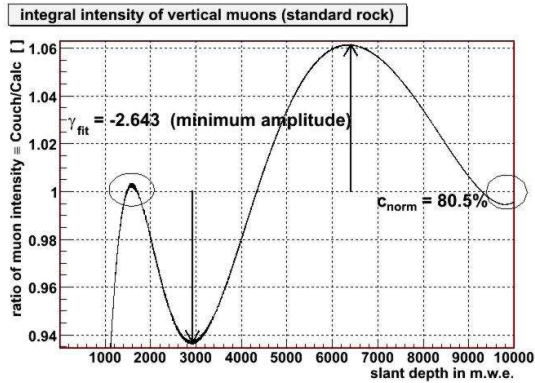
Figure 3: Fractional difference between the integral vertical muon intensity underground according to the Crouch curve and the optimized calculation for slant depth values in standard rock.
