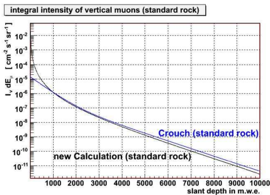
Figure 2: Calculated integral vertical muon intensity underground as a function of slant depth in standard rock in comparison with the Crouch function [6].
