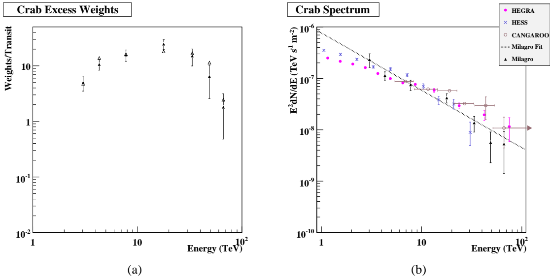
Figure 3: Preliminary results on the Crab energy spectrum. (a) Excess weights as a function of energy, with the number of expected weights computed for the fit spectrum shown to the right. (b) Comparison of the spectrum fit to Milagro data and other IACT experiments.
