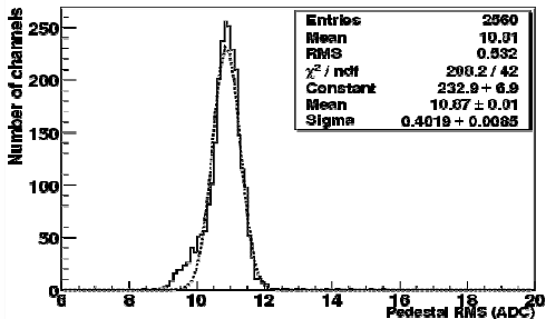
Figure 1. Pedestal RMS distribution of all 2560 channels.
