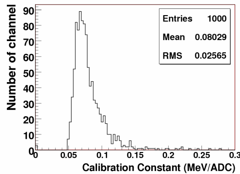
Figure 6. A distribution of calibration constants for the CREAM-III calorimeter.
