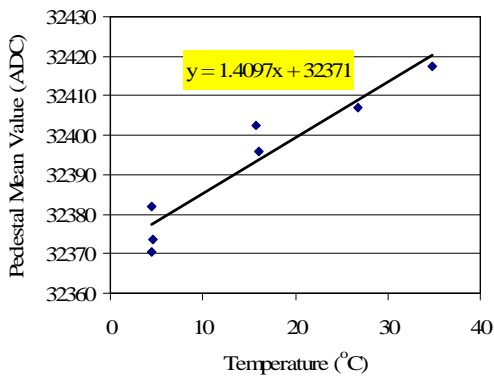
Figure 4. Pedestal mean value as a function of temperature showing a 1.4 ADC/°C slope.
