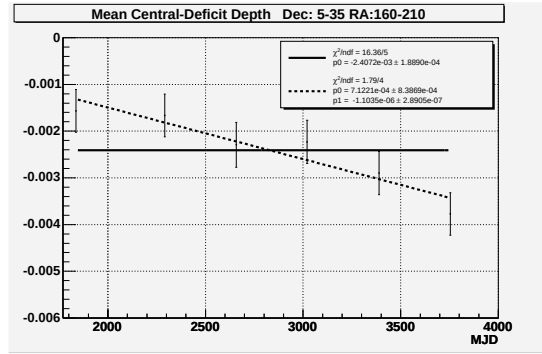
Figure 3: Mean depth of the central-deficit region vs. MJD for yearly sets from 2000-2006. The error bars are the stat. + sys. errors. The mean is taken from 5^\circ to 35^\circ in dec. and 160^\circ to 210^\circ in r.a. The solid line is the flat one-parameter fit and the dashed is the linear two-parameter fit. The \chi^2/\text{ndf} for the fits are 16.4/5 and 1.8/4 respectively.
