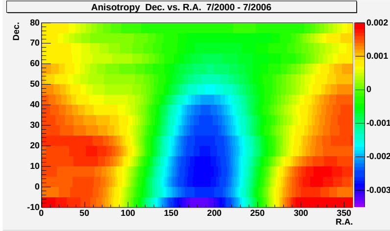
Figure 2: Fractional difference of the cosmic ray rates from isotropic in equatorial coordinates as viewed by Milagro for the years 2000-2006. The color bin width is 1.0 \times 10^{-4} reflecting the average measurement error. The median energy is 3 TeV.
