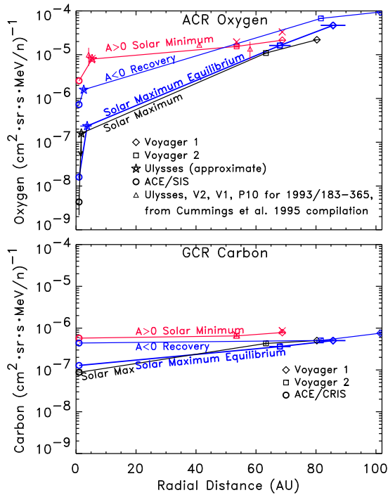
Figure 4: Intensity vs. radial distance for ACR oxygen ( top ) and GCR carbon ( bottom ) from ACE (circles), Voyager 1 (diamonds), Voyager 2 (squares), and Ulysses (stars) during the 4 periods of interest. Solar minimum values from an earlier study [1] (triangles) and without latitudinal gradient corrections (crosses) are also shown.
