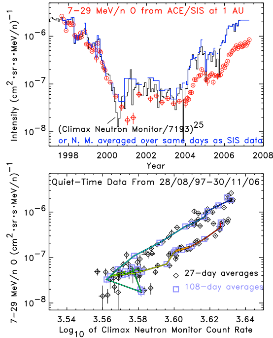
Figure 1: Top: Quiet time 7-29 MeV/nucleon oxygen from ACE/SIS (circles) compared with the Climax neutron monitor rate (black histogram) and the Climax rate during the same quiet days as used for the SIS data (blue histogram), both scaled as indicated. Bottom: ACE/SIS 7-29 MeV/nucleon oxygen vs. the Climax neutron monitor count rate.
