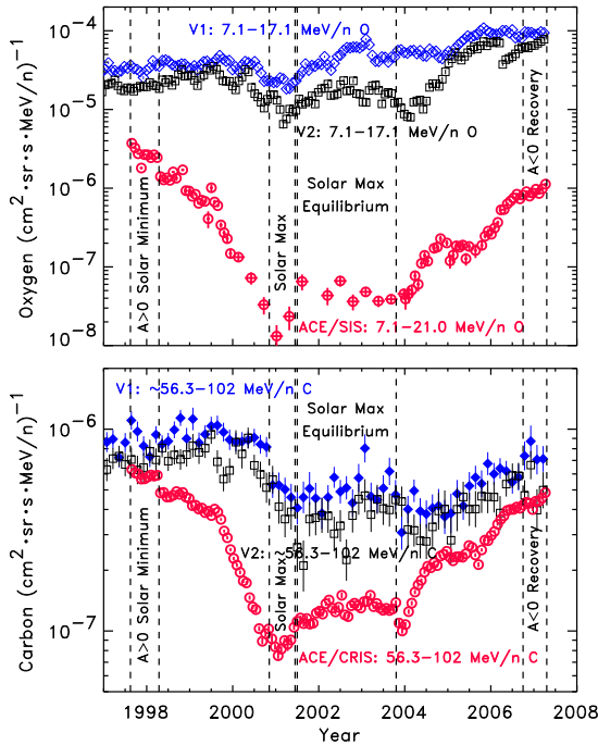
Figure 2: Oxygen intensity ( top ) (mostly ACRs, but with GCR background; see Figure 3) and GCR carbon ( bottom ) vs. time from ACE (circles), Voyager 1 (diamonds), and Voyager 2 (squares). The 4 time periods in which we determine the radial gradient are indicated between vertical dashed lines.
