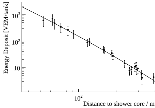
Figure 2: Signal vs distance from shower core with fitted lateral distribution for an event with an estimated energy of 100 PeV.
