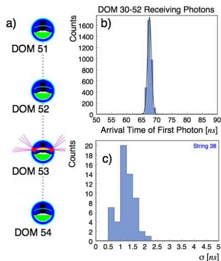
Figure 4: a) DOM 53 is flashing. b) Photon arrival time delay at DOM 52 when DOM 53 is flashing. c) RMS variation of time delay measured with flashers for 59 DOM pairs on an IceCube string.
