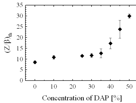
Figure 6: The detection threshold (Z/\beta)_{th} as a function of DAP concentration in copolymers.
