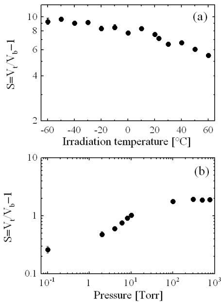
Figure 5: The variation of S in the CR-39 detector for irradiation, (a) temperature and (b) pressure.
