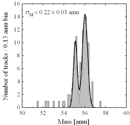
Figure 3: Mass distribution for iron nuclei in the CR-39 detector [8].
