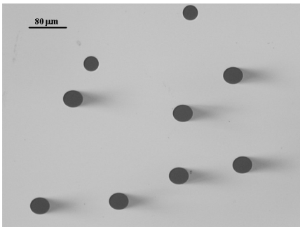
Figure 1: Microscopic image of etch pit of Fe ions produced in the CR-39 detector.
