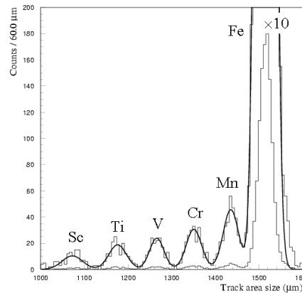
Figure 2: Track area distribution in the CR-39 detector. Nuclei lighter than Fe are seen as products of the fragmentation reaction.
