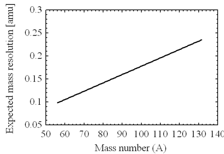
Figure 4: Variation of mass resolution expected for region 56 \leq A \leq 132 in the CR-39 detector [8].
