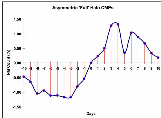
Fig 2: The results of Chree analysis of superposed epoch from -10 to +10 days with respect to zero epoch days for Asymmetric 'Full' Halo CMEs.
