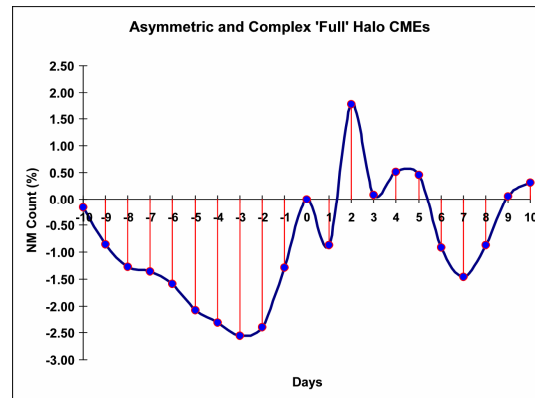
Fig 4: The results of Chree analysis of superposed epoch from -10 to +10 days with respect to zero epoch days for Asymmetric and Complex 'Full' Halo CMEs.
