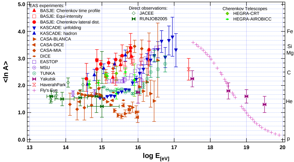
Figure 1: Mean logarithmic mass of primary cosmic rays
