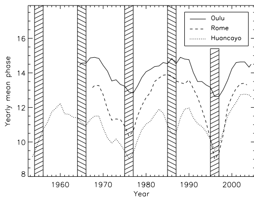
Figure 2: Yearly mean phases at Oulu, Rome, & Huancayo NM stations. The solid line stands for Oulu, the dashed line indicates Rome, and the dotted line represents the Huancayo NM station.
