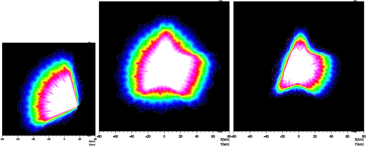
Figure 2: TA FD trigger functions at 10^{20} eV for observation modes of mono station, mono/3 stations (OR sum of the three mono trigger functions), and stereo/3 stations (OR sum of the stereo trigger functions of {}_3C_2 combinations).
