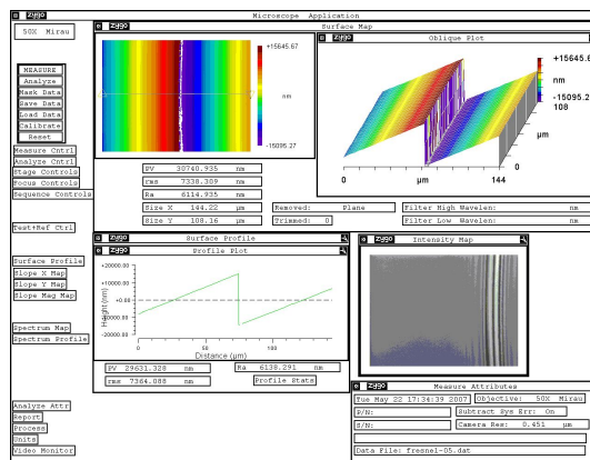
Figure 5: Measurement of fresnel structure of the fig.4.
