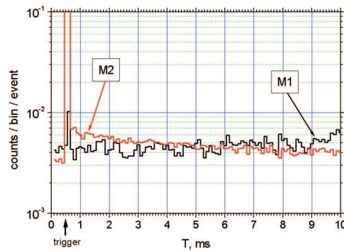
Figure 2: Pulse delay distributions measured by the ZnS detector for different triggers.
