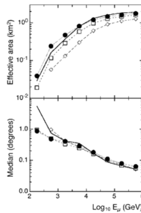
Figure 3: Effective areas and median angles between true and reconstructed muon tracks as a function of muon energy for different detector configurations. The solid line is for the 10x10 “homogeneous” detector with a 20 kHz background. Symbols are for a 9x9 array of “NEMO Towers” with different background rates: 20 kHz (full dots), 60 kHz (open squares) and 120 kHz (open diamonds).
